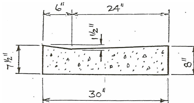
TYPICAL DRIVEWAY CURB CUT
